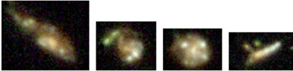
Fig. 4 Distant galaxies from the Hubble Deep Field. The distorted appearances of these galaxies suggest that they collided with other galaxies shortly before their light began the long journey to Earth.
